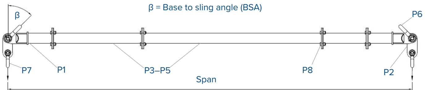
Fig.1 Typical Spreader Assembly
