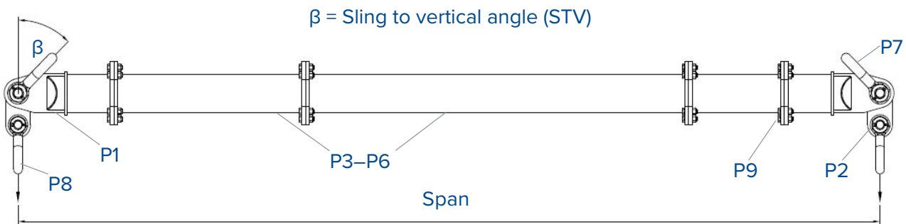
Fig.1 Typical Spreader Assembly
