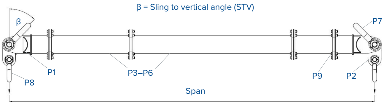
Fig.1 Typical Spreader Assembly
