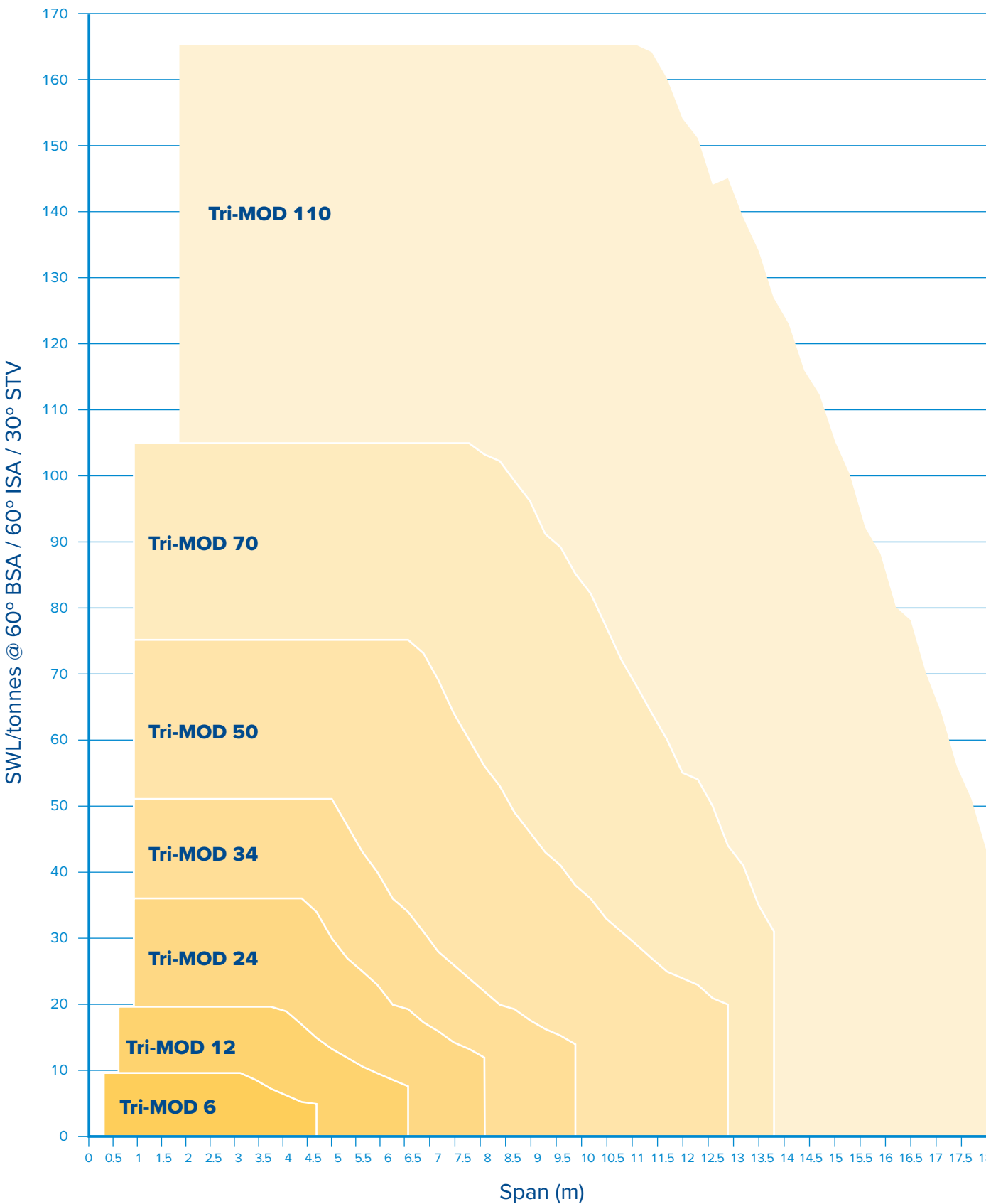
Load v span chart TriMOD 6 to 110
