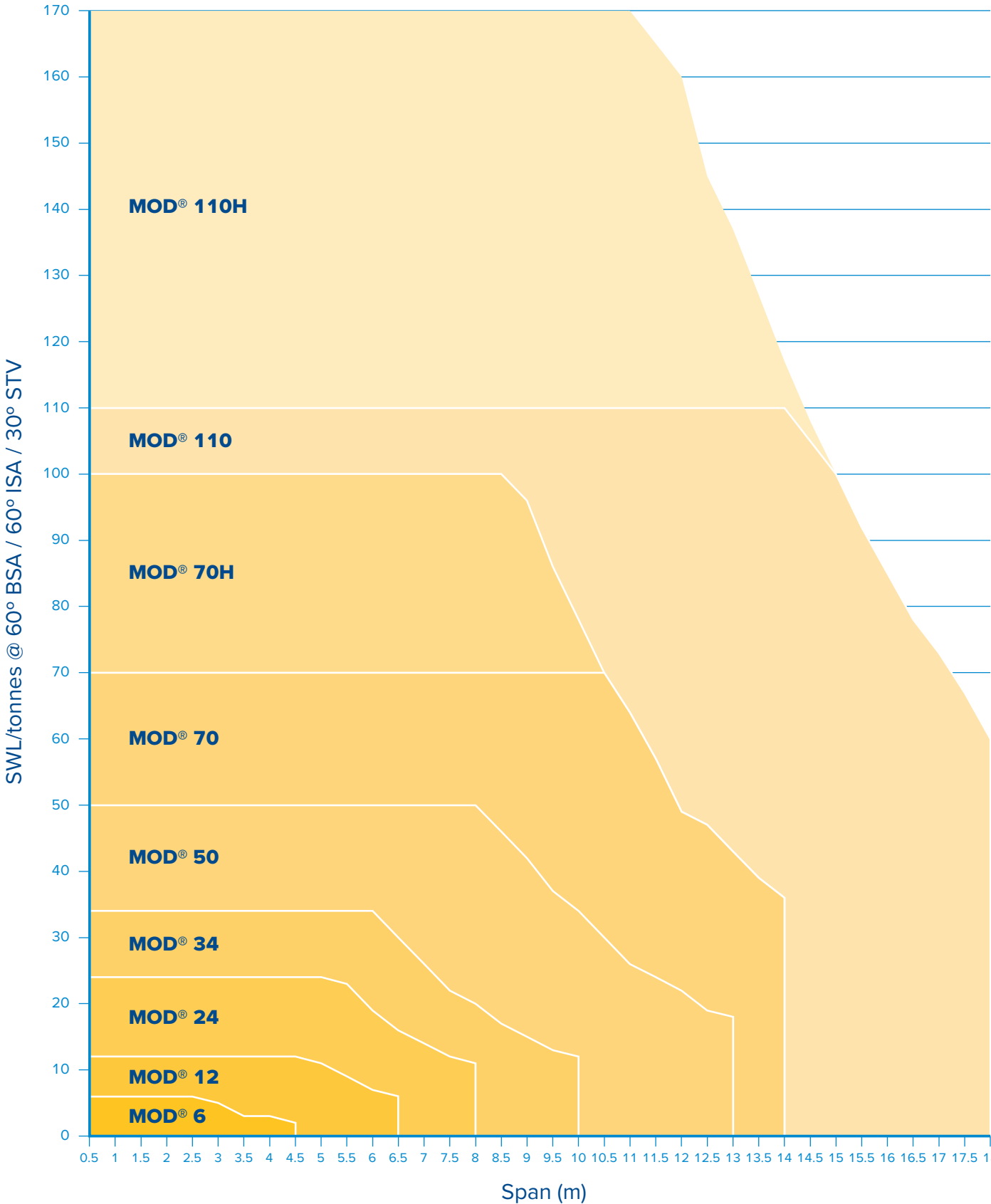
Load v span chart MOD ® 6 to 110H
