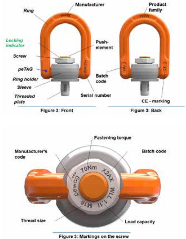
Fig. 3: Component descriptions and location of the identification details on the product.
