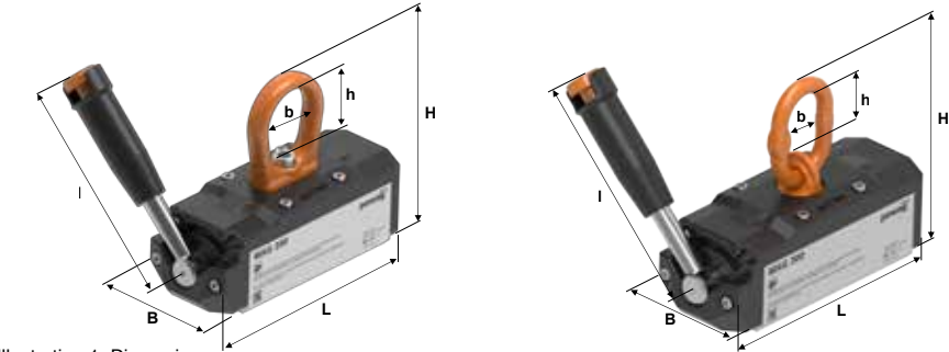
Illustration 1: Dimensions
